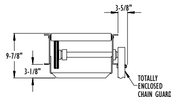
SECTION "Y-Y"
